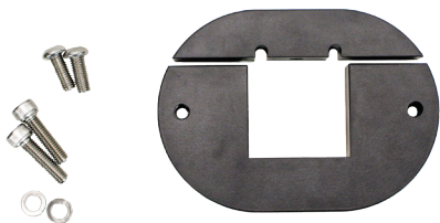
2" x 2" Roll Bar Mounting Bracket PN: 2632
